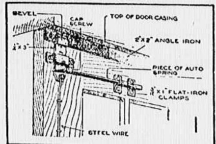
Scraps of Bar Iron and an Old Auto Spring Are Made Into an Unusually Durable Garage-Door Latch.
