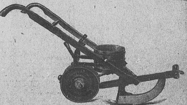
COLE PLAIN-VIEW CORN PLANTER NO. 11, PRICE $12.50
