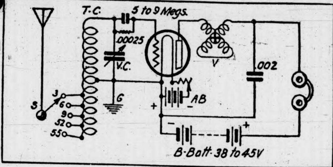
Diagram That Introduces a New Field of Selectivity Into the Multi-Audi-Plex Circuit. Will Interest All Radio Fans.
