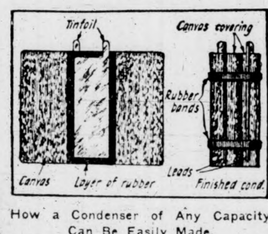
How a Condenser of Any Capacity Can Be Easily Made.
