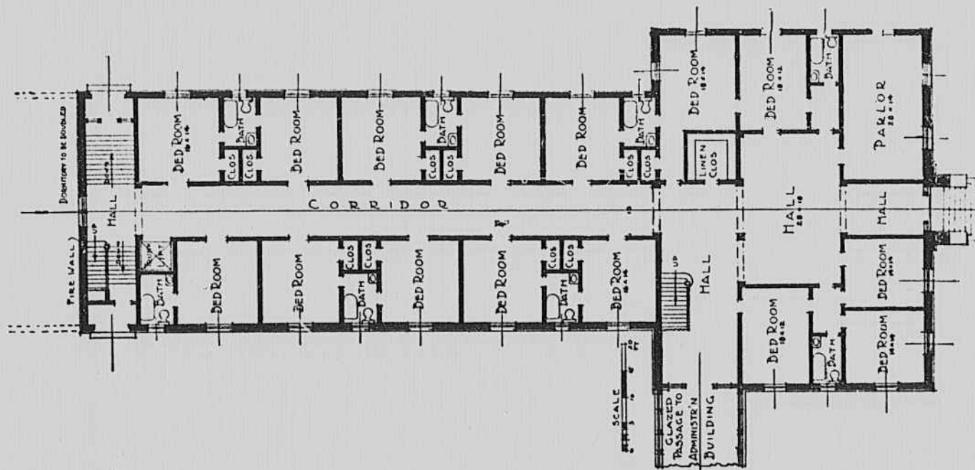
Ground Floor of a Dormitory. Both floors of each dormitory are practically the same.
